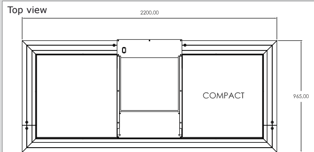
Smoking cabin Compact
